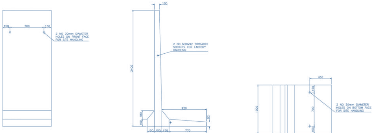
Figure 2 – Dimensions for 3000 Retainer Wall Unit
