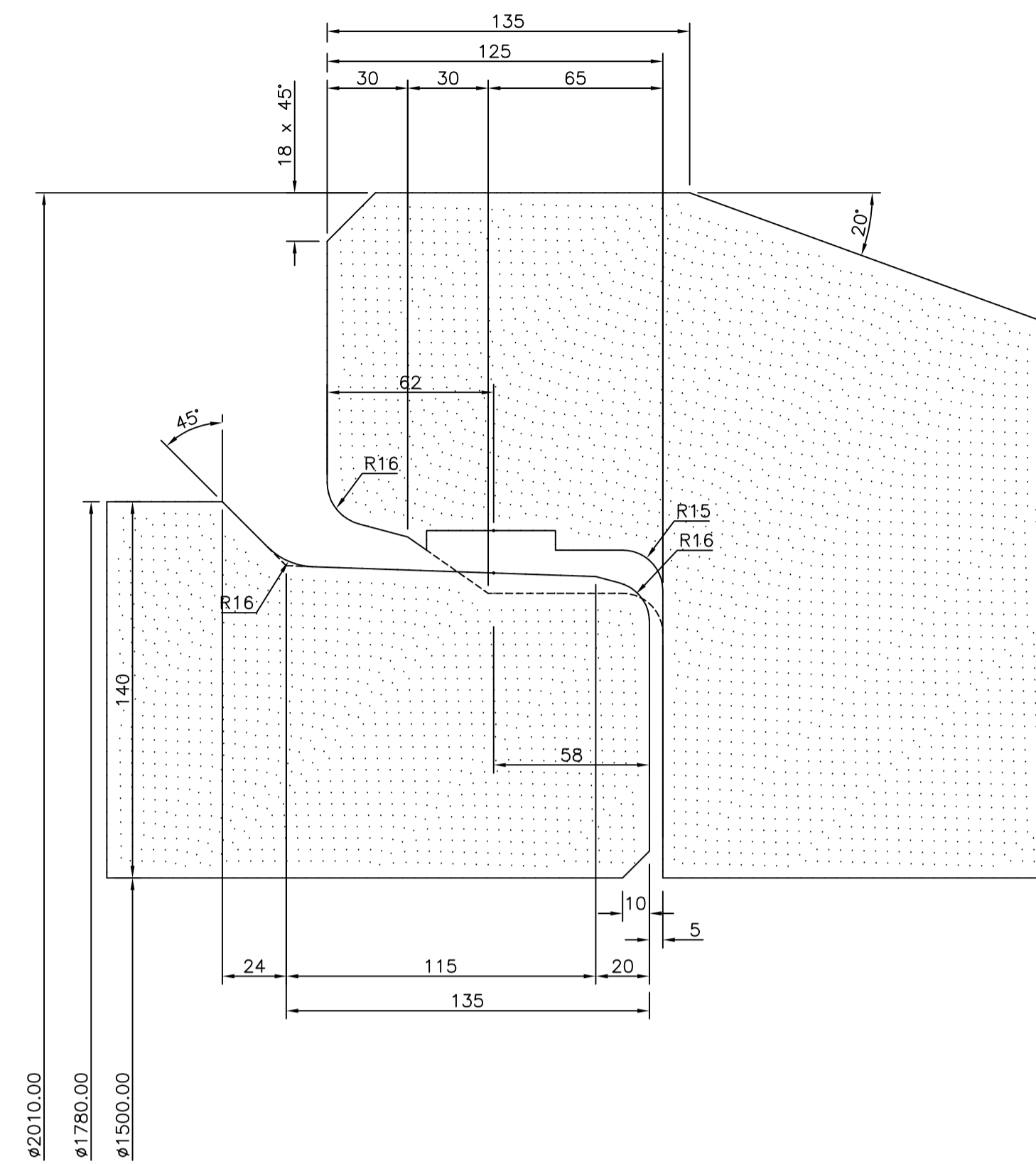
DETAIL SCALE 1:2
